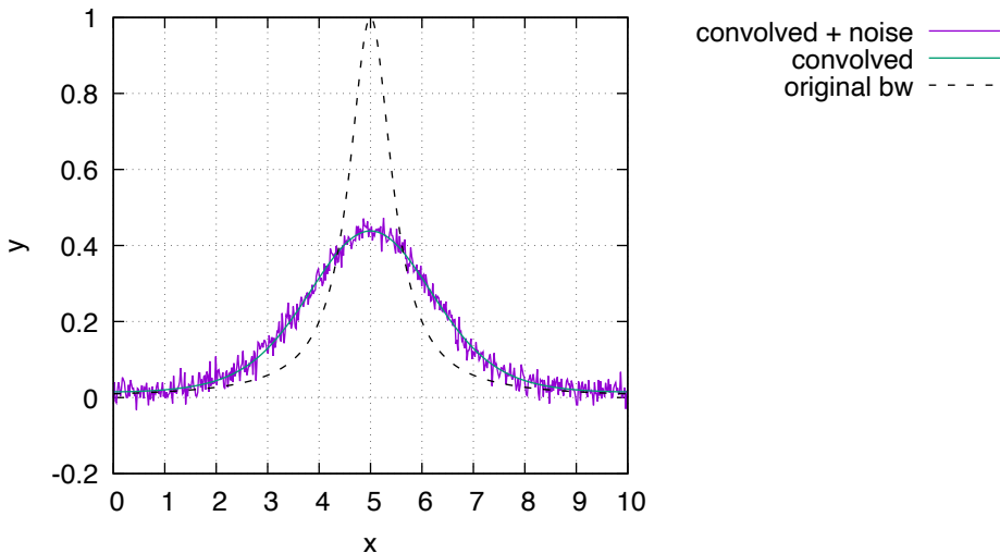
Convolved noisy breit wigner signal
